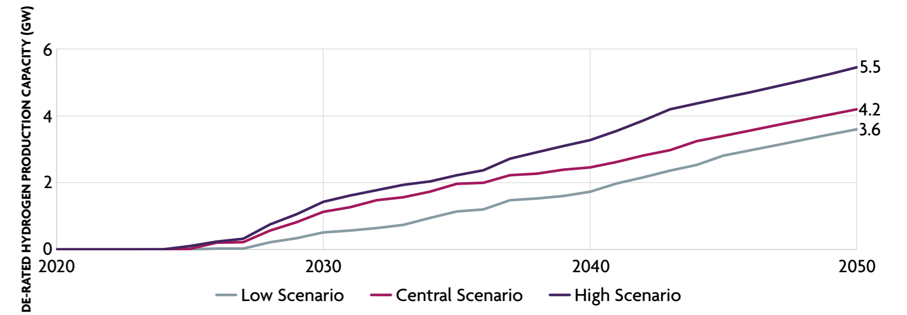
DE-RATED HYDROGEN SUPPLY TO SUPPORT DEMAND IN NORTH WEST ENGLAND AND NORTH WALES
