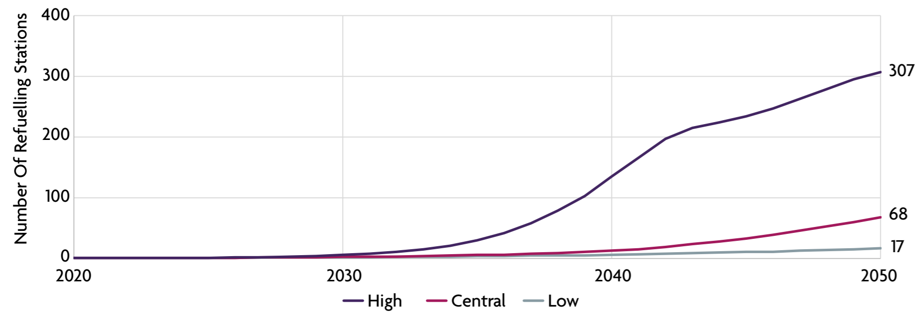
NUMBER OF 2T/DAY HYDROGEN REFUELLING STATIONS AT 80% UTILISATION
