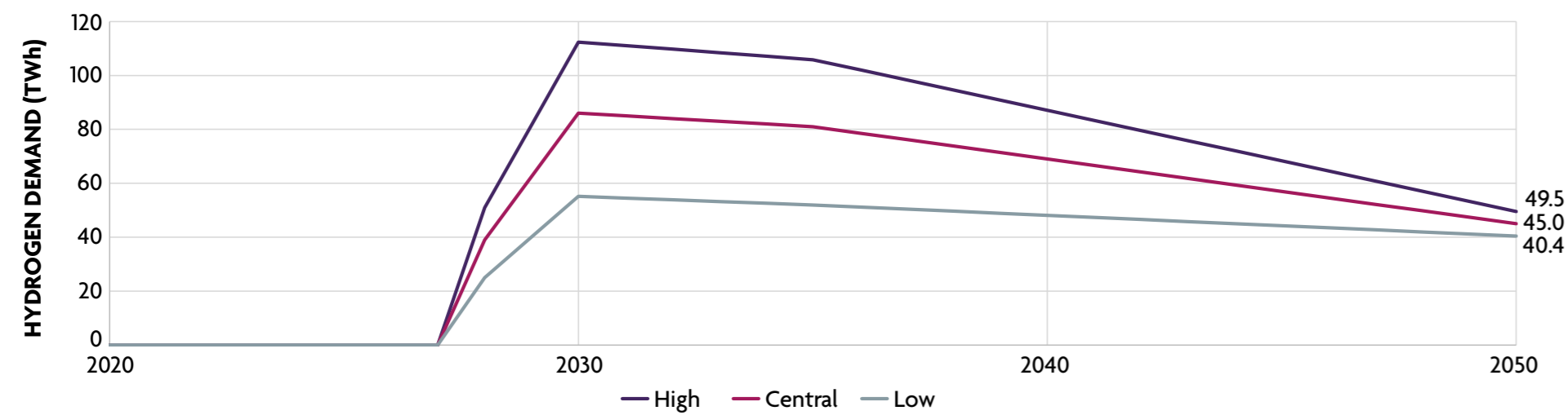
HYDROGEN DEMAND FOR POWER IN GREAT BRITAIN
